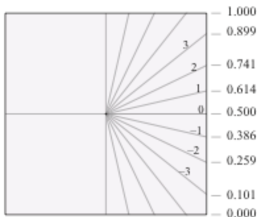
Figure 28. Intersections of seventh angular divisions with the edge of the paper.
