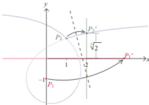
Figure 36. Another folding sequence to construct \sqrt[3]{2} .
